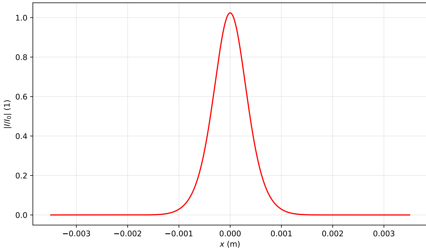
Intensity profile I(x, y = 0, z = 1.194)/I_0 , P_{in}=0.5P_{cr} , artificial time
